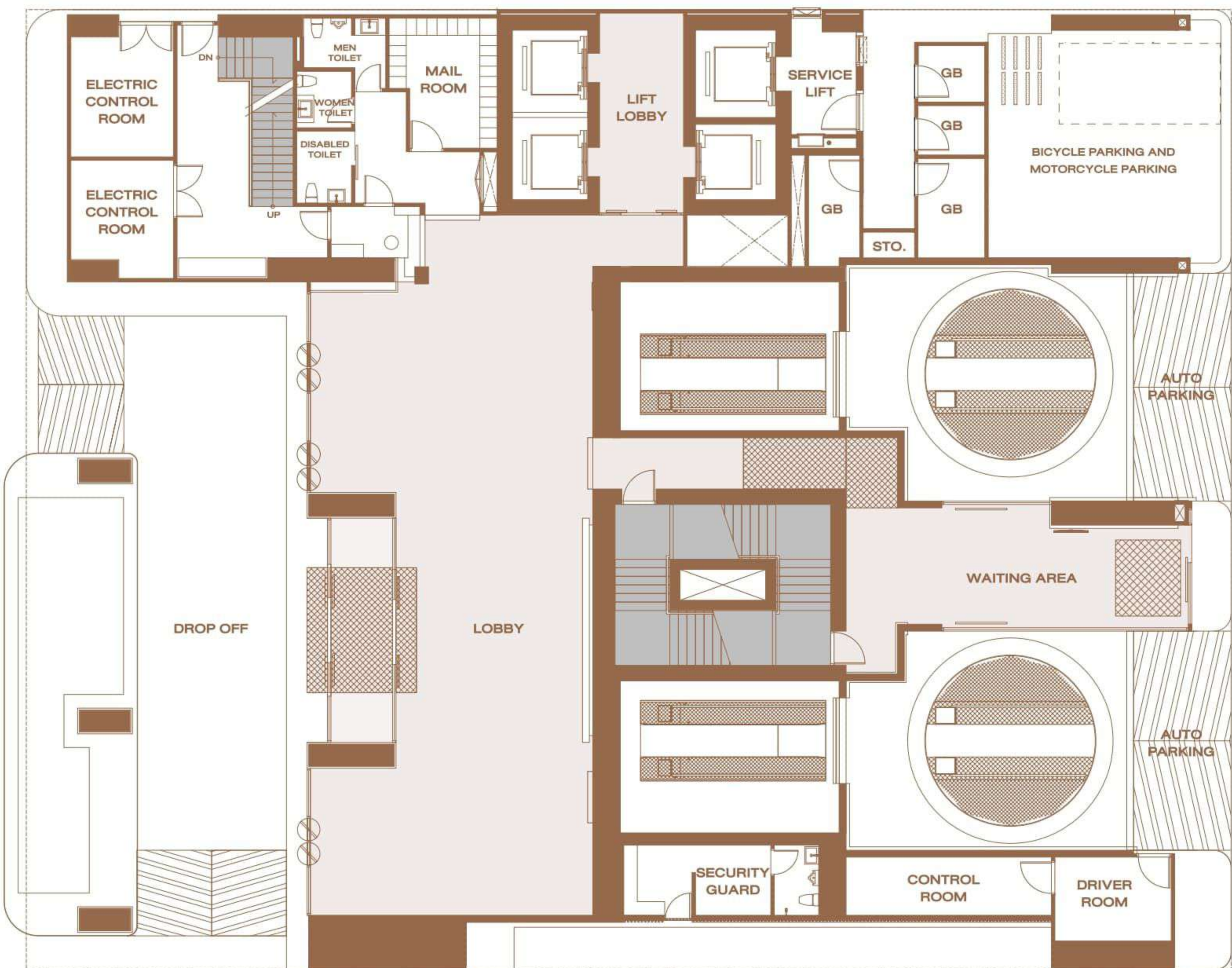
1 st FLOOR
